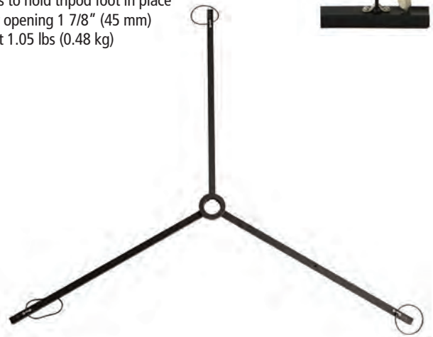
5610-01 — Tripod Stabilizer
